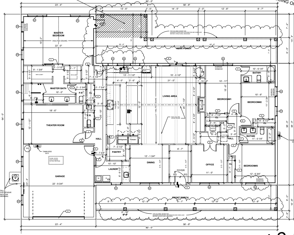
1 FLOOR PLAN 1/8" = 1'-0"
